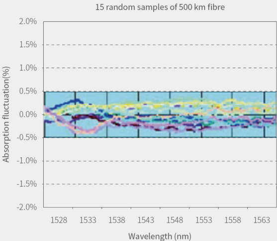
Absorption Reproducibility (+/- 0.3% in the C Band)
